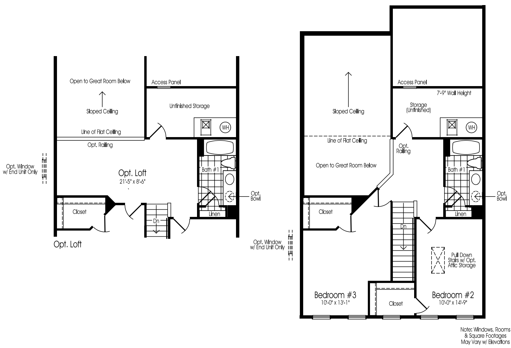
UPPER LEVEL ELEVATION A
